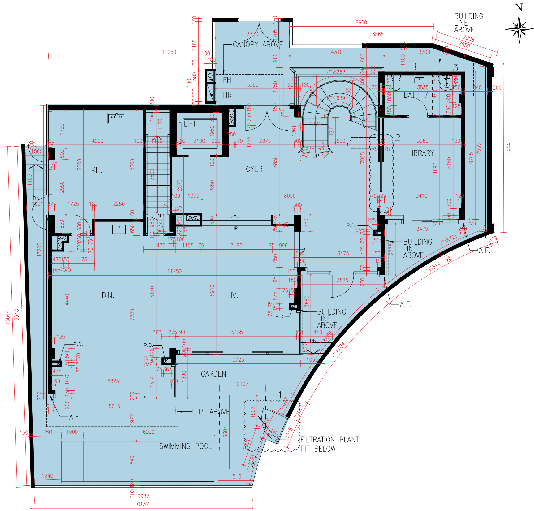
GROUND FLOOR PLAN (showing the "as-is" condition) 地下平面圖 (顯示「現狀」)
