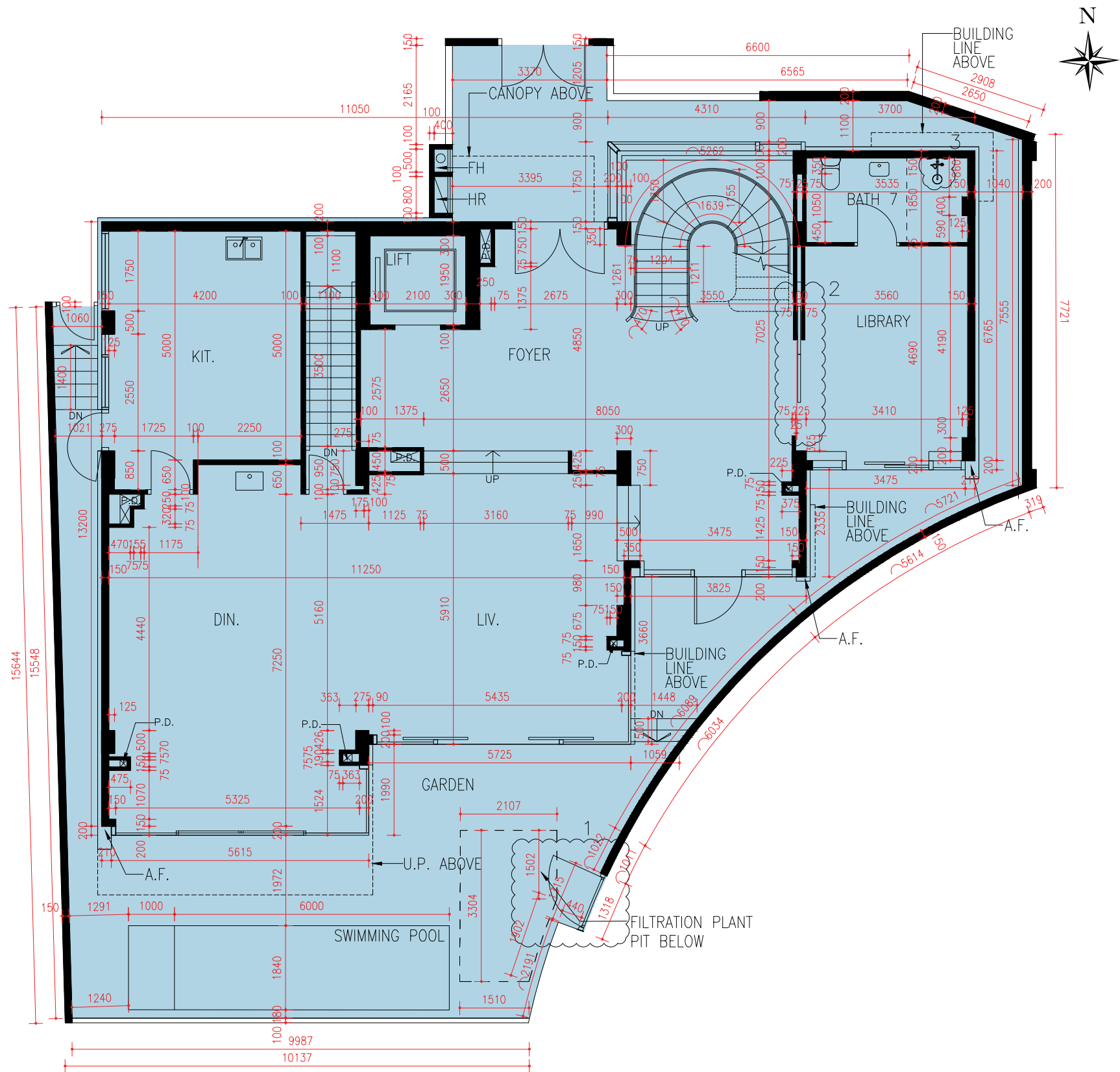
GROUND FLOOR PLAN (showing the "as-is" condition)
